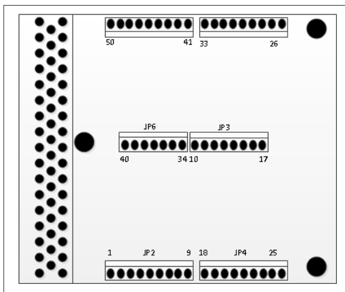
Figure 14 Y1180A 50 Pin Shielded Connector Block PC Board
