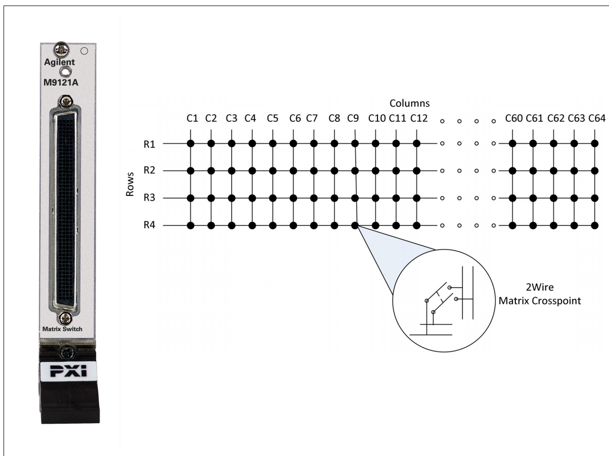
Figure 10 M9121A Front Panel and Simplified Schematic
