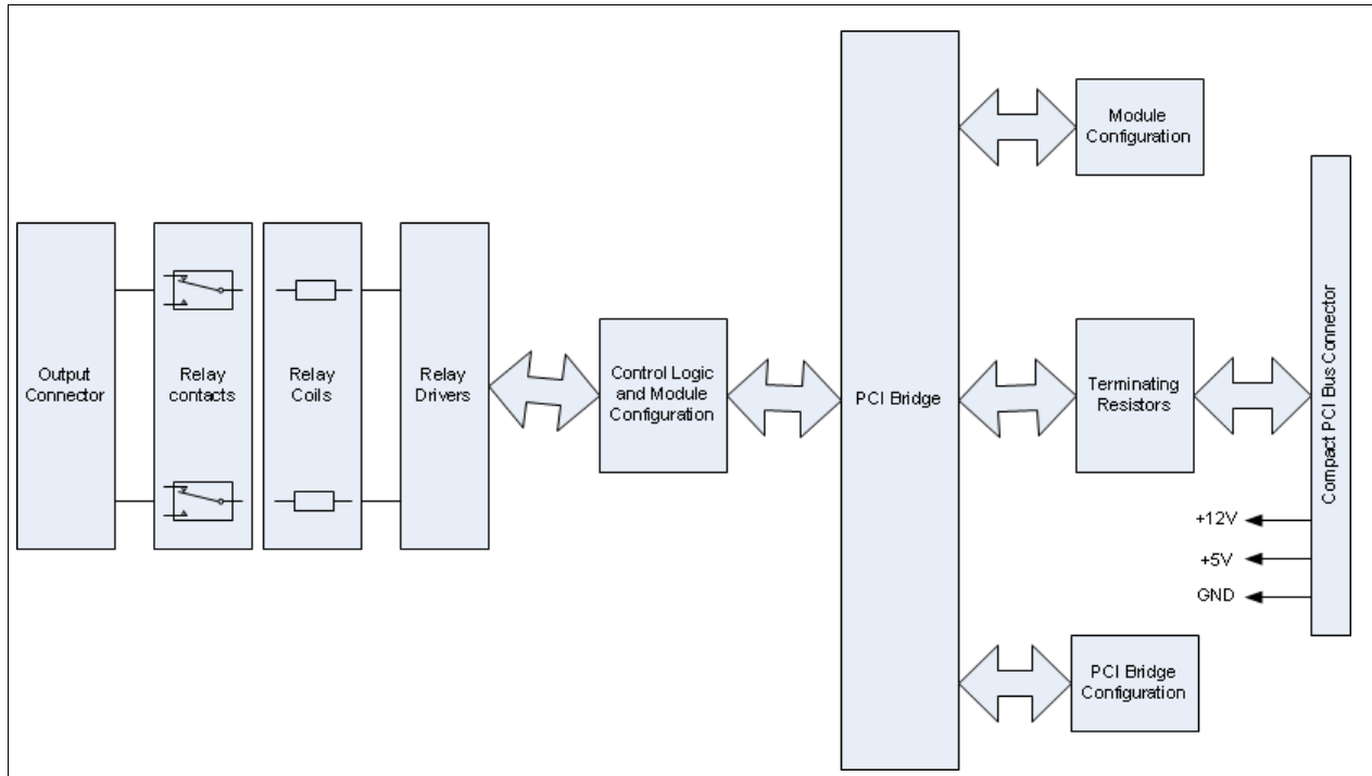
Figure 1 PXI Matrix and Multiplexer Switch Module Functional Block Diagram
