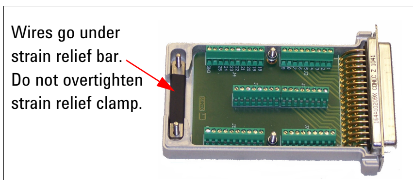
Figure 22 Using the Strain Relief Clamp
