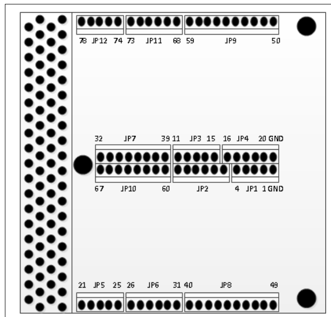
Figure 15 Y1181A 78 Pin Shielded Connector Block PC Board
