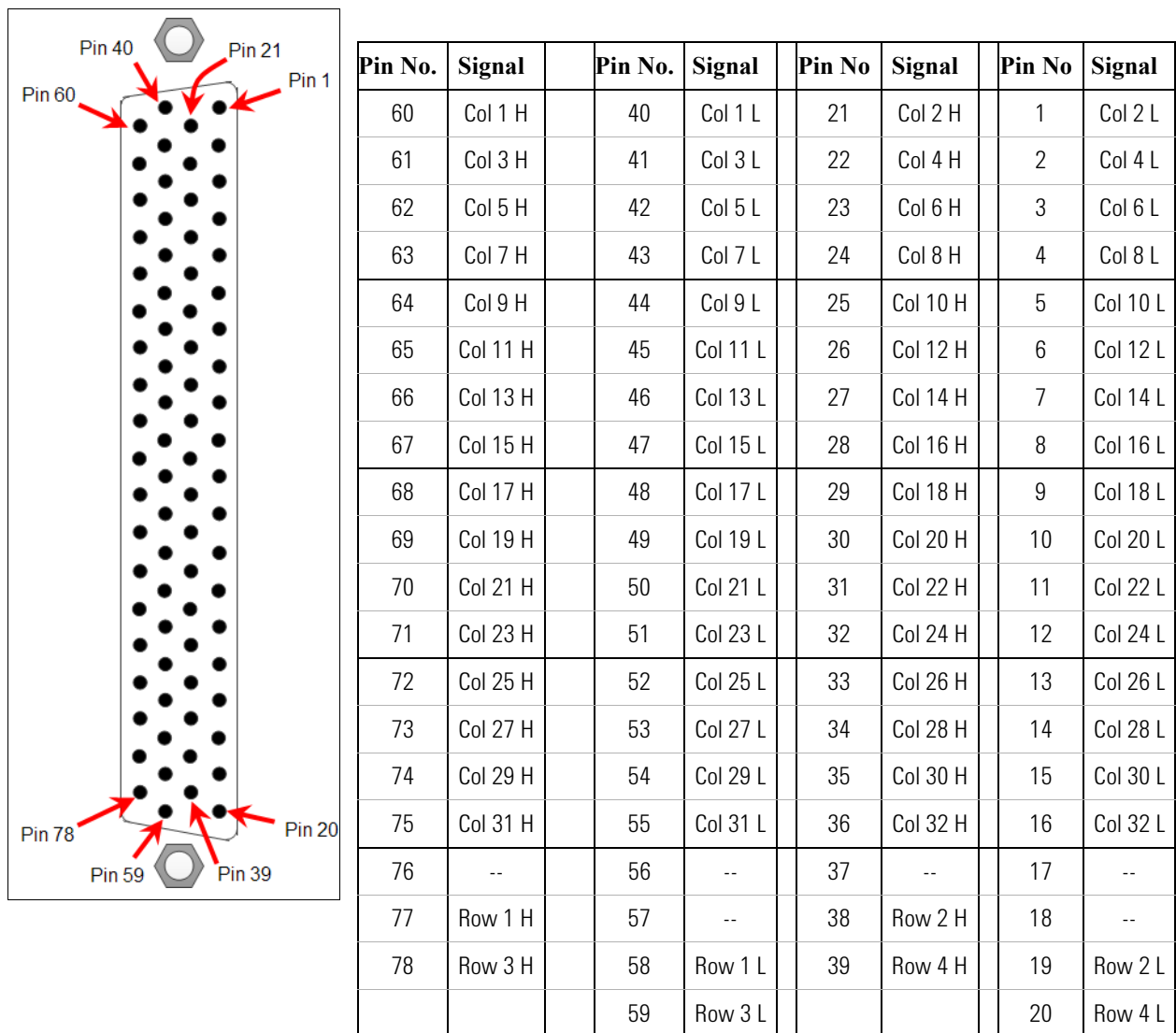
Figure 9 M9120A Connector (viewed from the front panel) and Pinout
